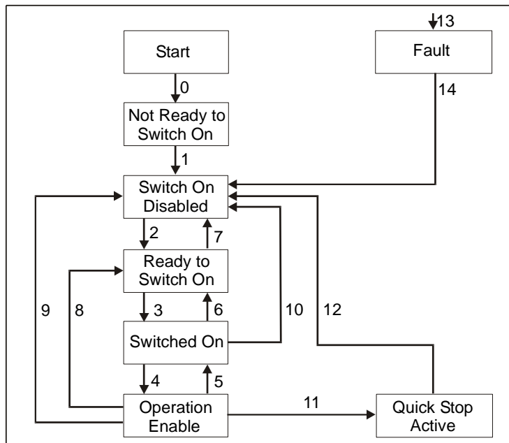
Fig. 10: State machine
