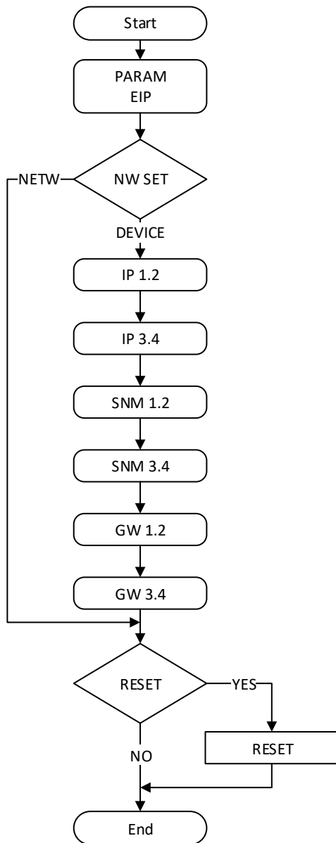
Fig. 16: Setting of the IP address
